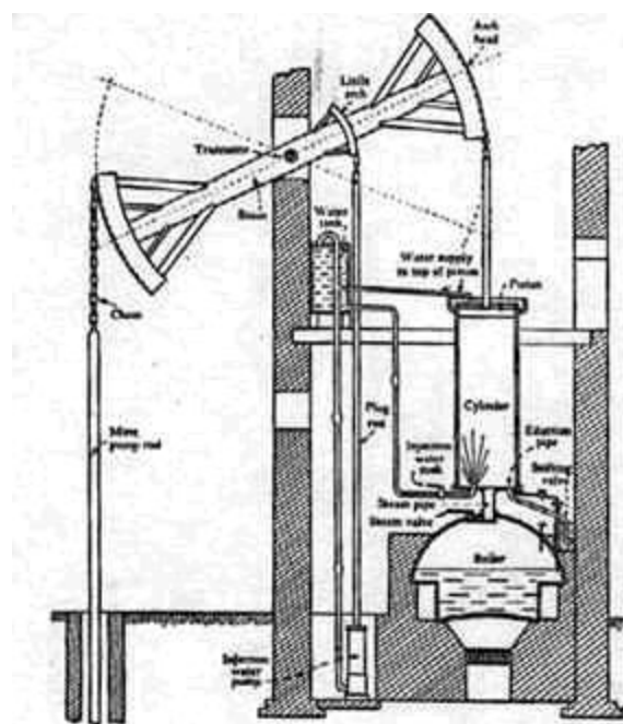
FIGURE 104—Diagram of Newcomen's atmospheric engine, 1712.
